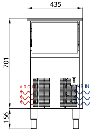
FRONTAL VIEW
