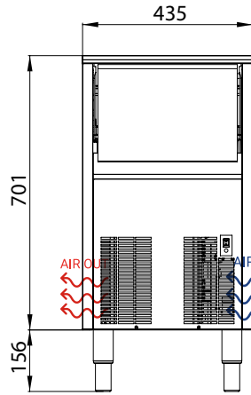
FRONTAL VIEW
